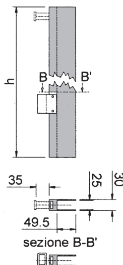
Posteriore Rear
